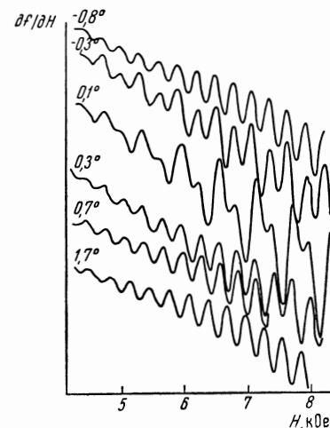
FIG. 5. Plots of the \alpha -oscillations of sample 2 when the field is rotated along the line aa; \mathbf{E} \parallel [010] , T = 1.3^\circ\text{K} , f = 5.0 Mcs. The curves are labeled with approximate values of the angle \varphi . (The angles were measured with approximate accuracy 10' , and the position \varphi = 0^\circ was determined from the symmetry of the effect.)
