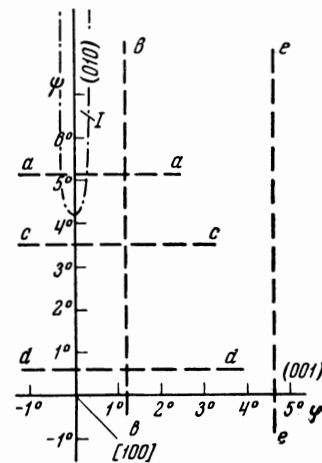
FIG. 3. Rectangular projection of the vicinity of the [100] axis on the direction sphere.
