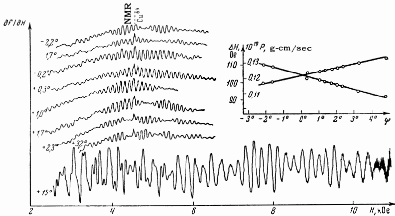
FIG. 6. Plots of the oscillations in sample 1, with the field rotated along the line bb and with polarization E \parallel [001] ; T = 1.3^\circ\text{K} , f = 5.1 Mcs. The curves are marked with the values of the angle \psi . In the right side of the lower curve are seen the quantum oscillations of the impedance [15] . The relative nuclear magnetic resonance amplitudes and the amplitudes of the quantum oscillations are reduced by several times compared with the amplitude of the oscillations of the size effect, owing to a large rate of change of the field during the time of recording.
