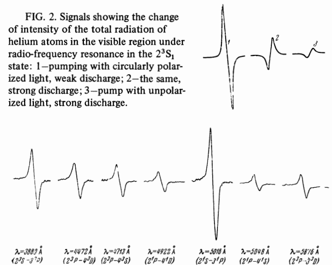
FIG. 3. Signals showing variation of the intensities of certain spectral lines of helium atoms emitted by the cell under radio-frequency resonance in the 2^3S_1 state. Pumping with circularly polarized light, weak discharge.
