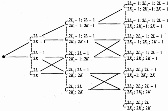
Fig. 1. Relation between various terms C_{\dots} . Dashed lines represent scattering process
